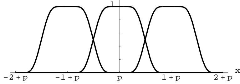
Fig.A1: A function \varphi(x) decomposing unity.
